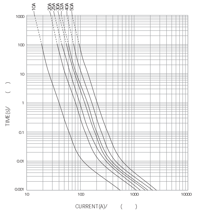
HC140EV-T I-T ( ) AVERAGE I-T CHARACTERISTICS CURVE (FOR REFERENCE ONLY)
